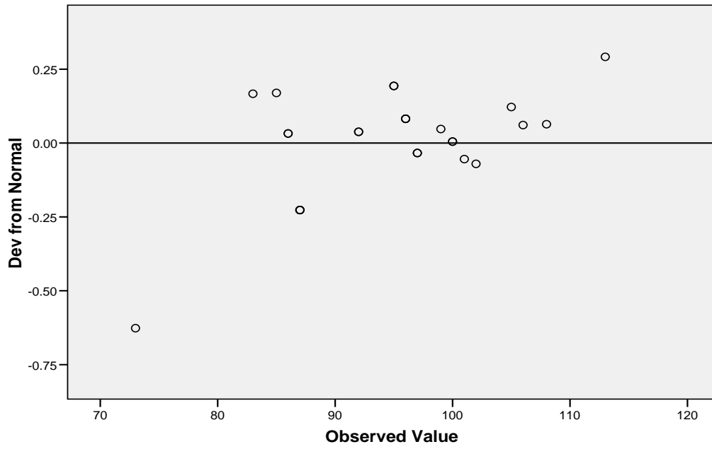
Detrended Normal Q-Q Plot of adversity_quotient
