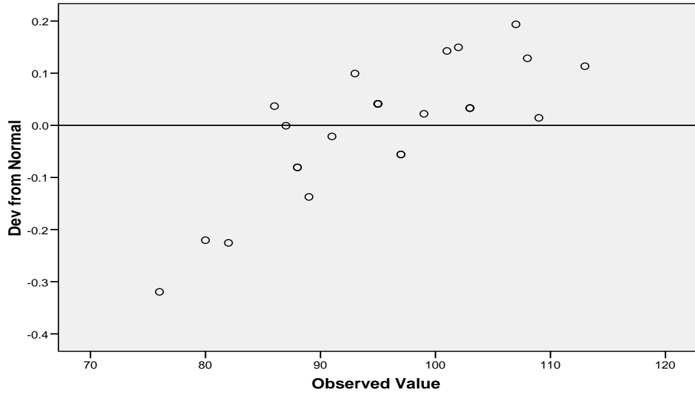
Detrended Normal Q-Q Plot of motivasi_belajar_PAI
