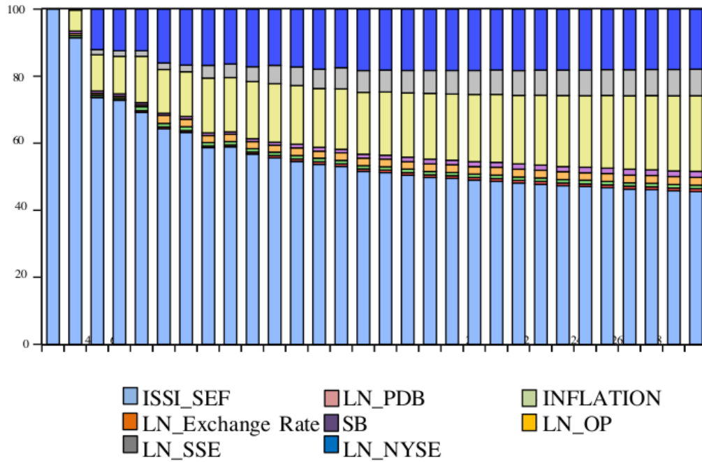
Picture 2. FEVD Results of Research Model 1
