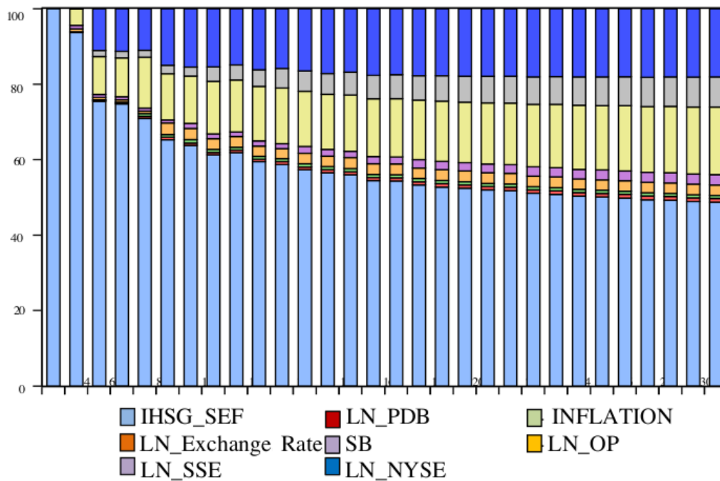
Picture 3. FEVD Results of Research Model 2
