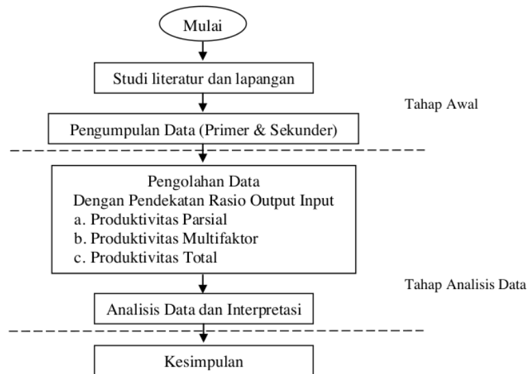
Gambar 1. Flowchart Penelitian
