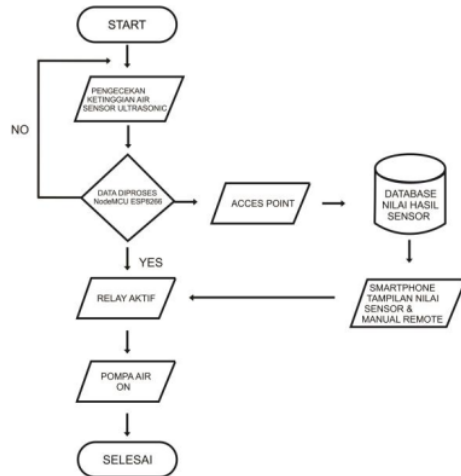
Gambar 6. Flow Chart
