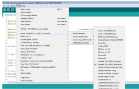
Gambar 16. Tampilan Program
