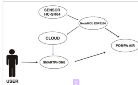
Gambar 8. Use Case
