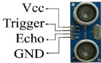
Gambar 2. Sensor HC-SR04
