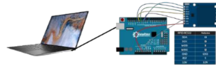
Gambar 4. Prototype Alat
