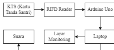
Gambar 3. Diagram Blok
