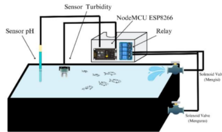
Gambar 2 Desain Prototype
