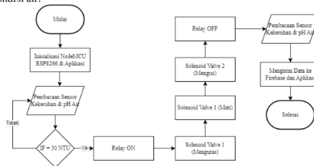
Gambar 1 Flowchart Sistem
