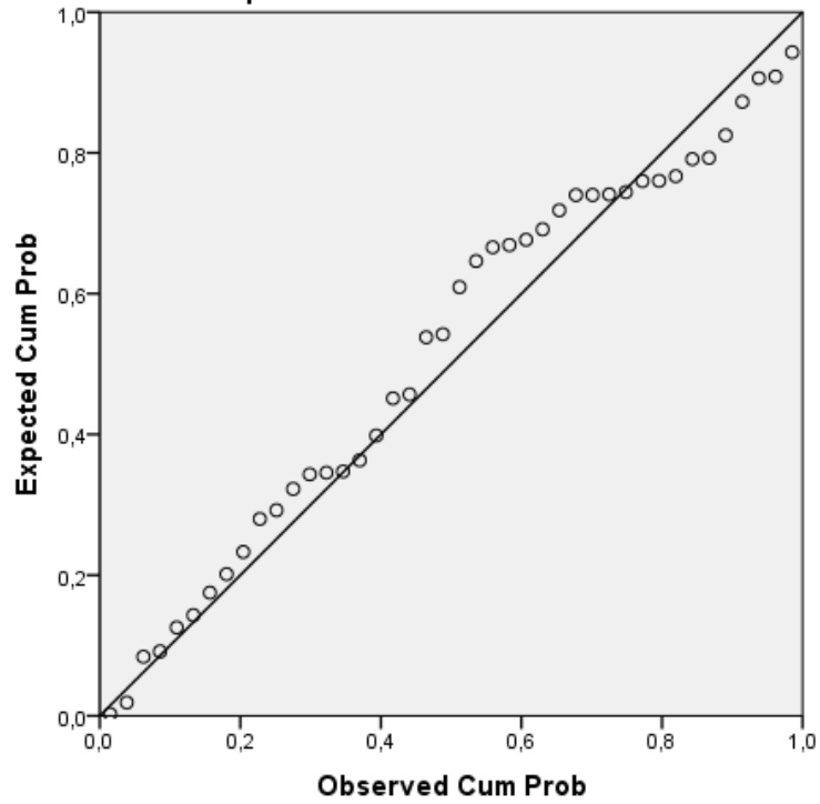
Normal P-P Plot of Regression Standardized Residual Dependent Variable: PROD
