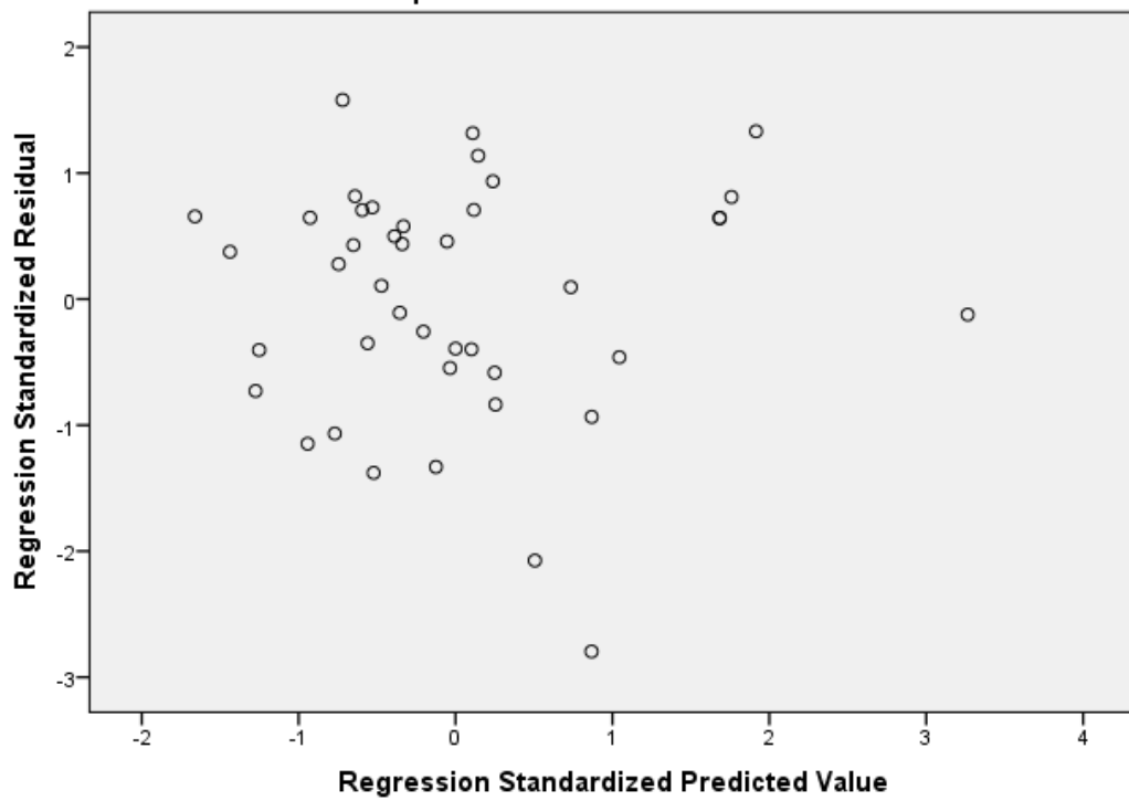
Dependent Variable: PROD
